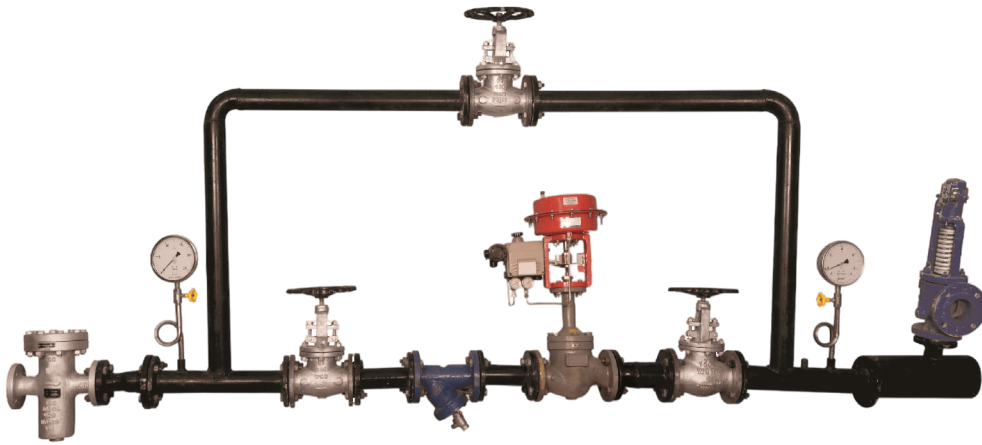
Pressure Reducing Station With Pressure Transmitter And PID Controller
