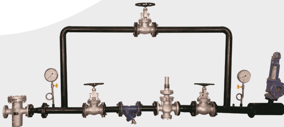
Pressure Reducing Station With Pilot Operated PRV
